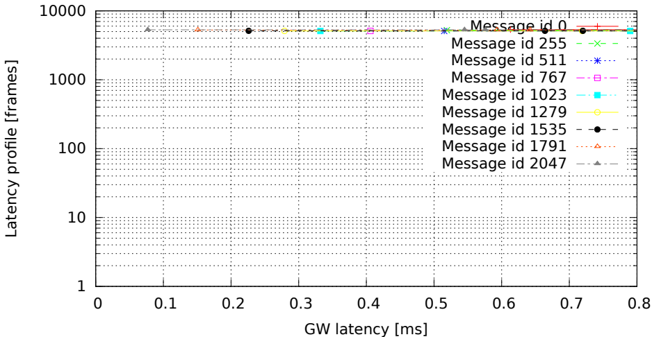
2048 GW rules (one per id, mask 0x7FF), no modifications (GW kernel 2.6.33.7-00007-g9c0ff90, Traffic 50, Load cpu)
